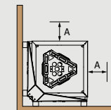
Corner Installation with Protective Cover
