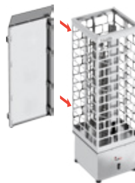
Wall Installation with Protective Cover
